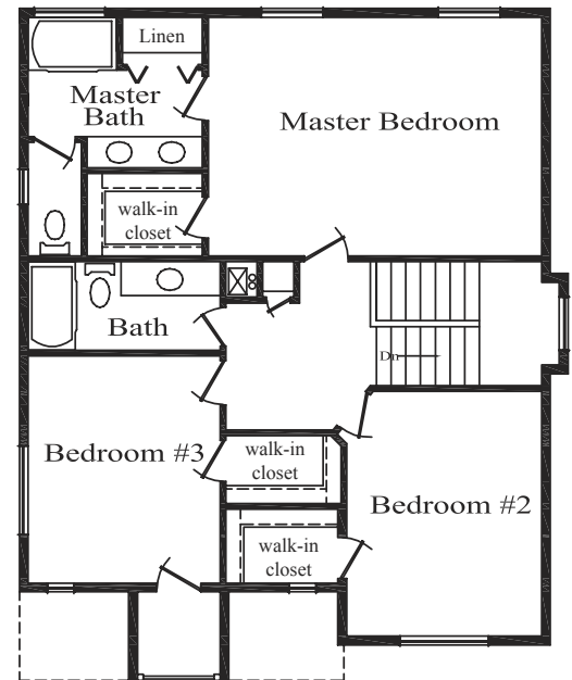
2nd Floor 1032 sq. ft.
