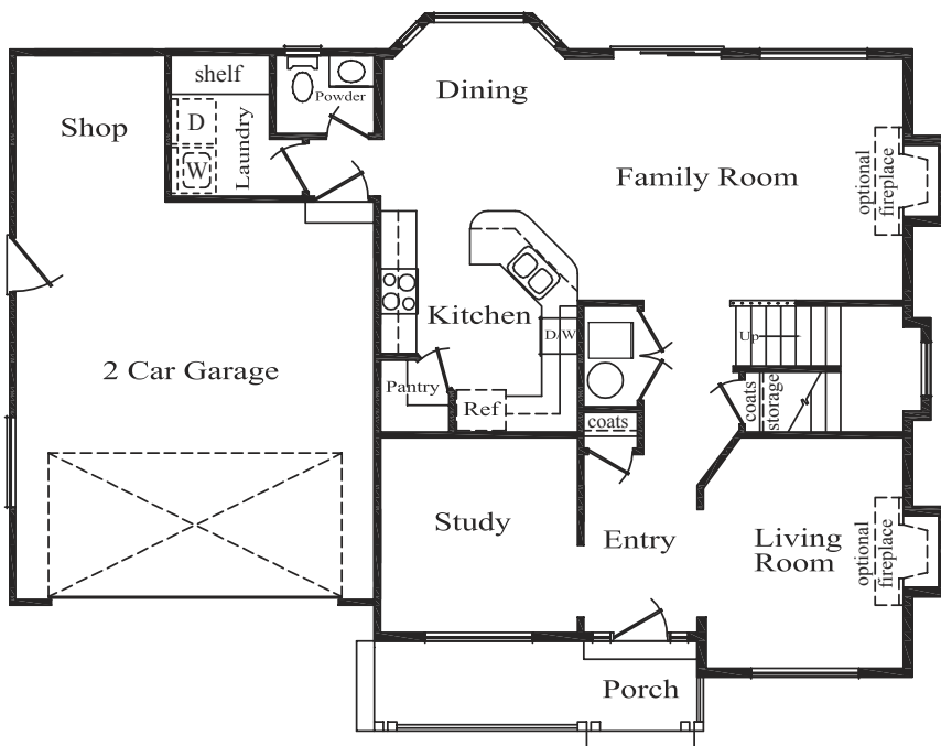
Main Floor 1155 sq. ft.
